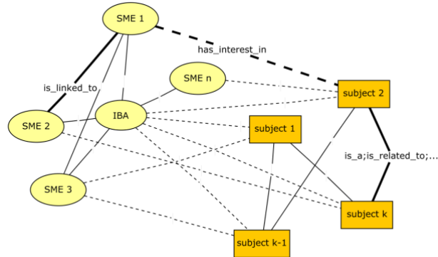
Fig. 2. Socio-semantic network model of a collaborative network mediated by the IBA-SME digital platform
