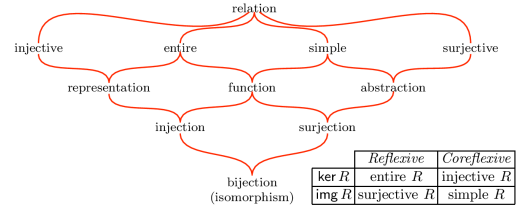
Figure 3: Binary relation taxonomy
