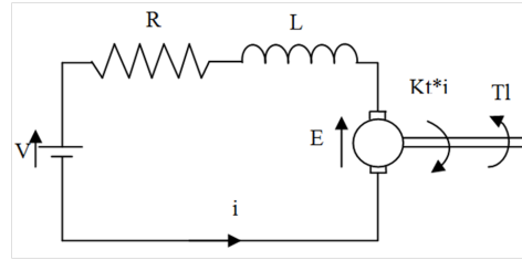
Fig. 8. schematic of the model
