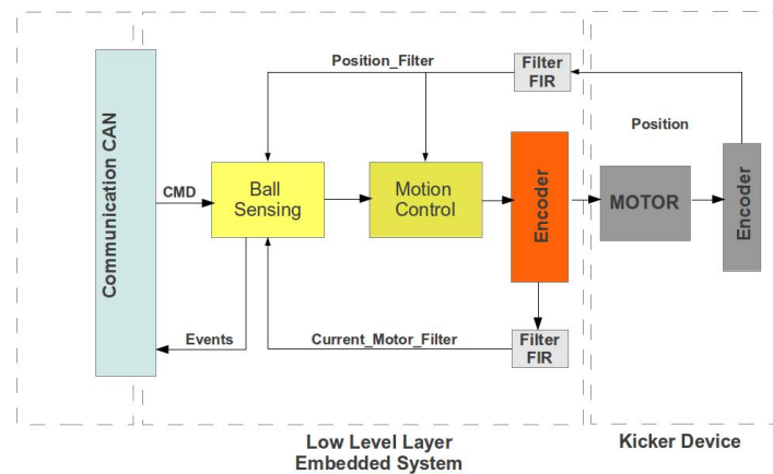
Fig. 9. Kicker Sensing implemented Architecture
