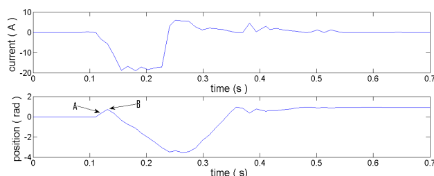
Fig. 3. kick with current detection system
