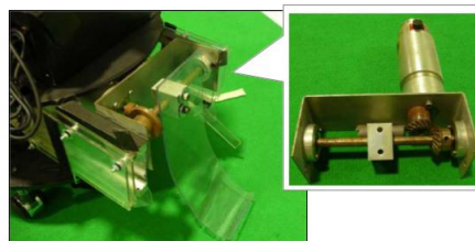
Fig. 2. Kicker Device
