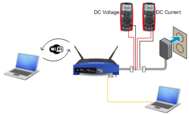
Fig 4 – Testbed
