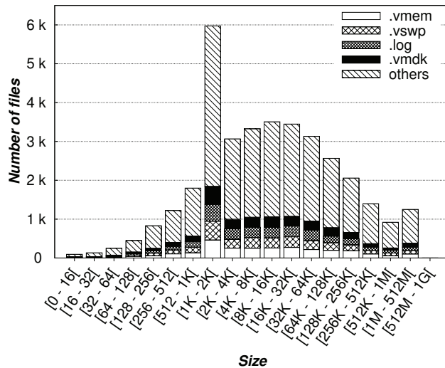
Fig. 7: Distribution of file sizes and extensions for the dataset used in §V ( others aggregates extensions other than .vmem , .vswp , .log , and .vdmk ).
