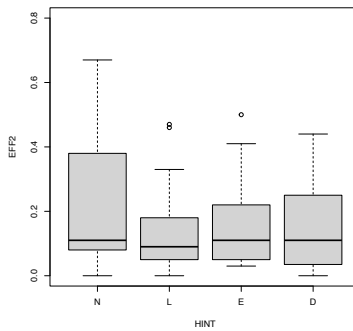
(e) Box-plot for EFF 2
