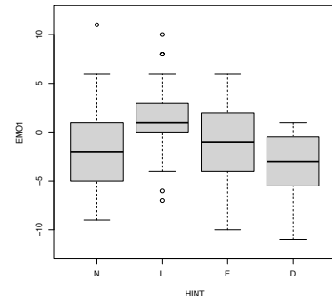
(c) Box-plot for EMO 1
