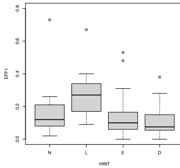
(b) Box-plot for EFF 1
