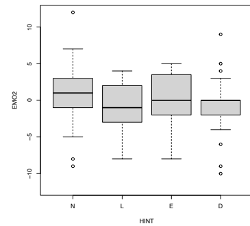
(f) Box-plot for EMO 2
