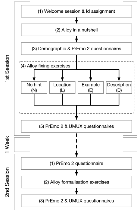
Figure 1: Overview of the experimental procedure
