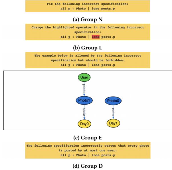
Figure 3: Treatment groups for task #1 of the 1st session
