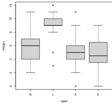
(a) Box-plot for PROD 1
