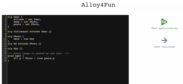
Figure 2: Alloy4Fun landing page with task #1 of the 1st session (treatment, i.e., hint message, omitted)
