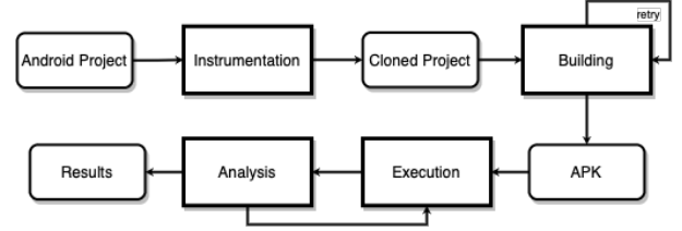
Fig. 1. PyAnaDroid default workflow
