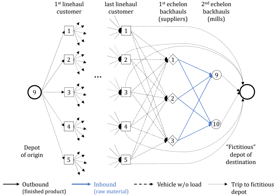
Figure 2: Network representation of the problem
