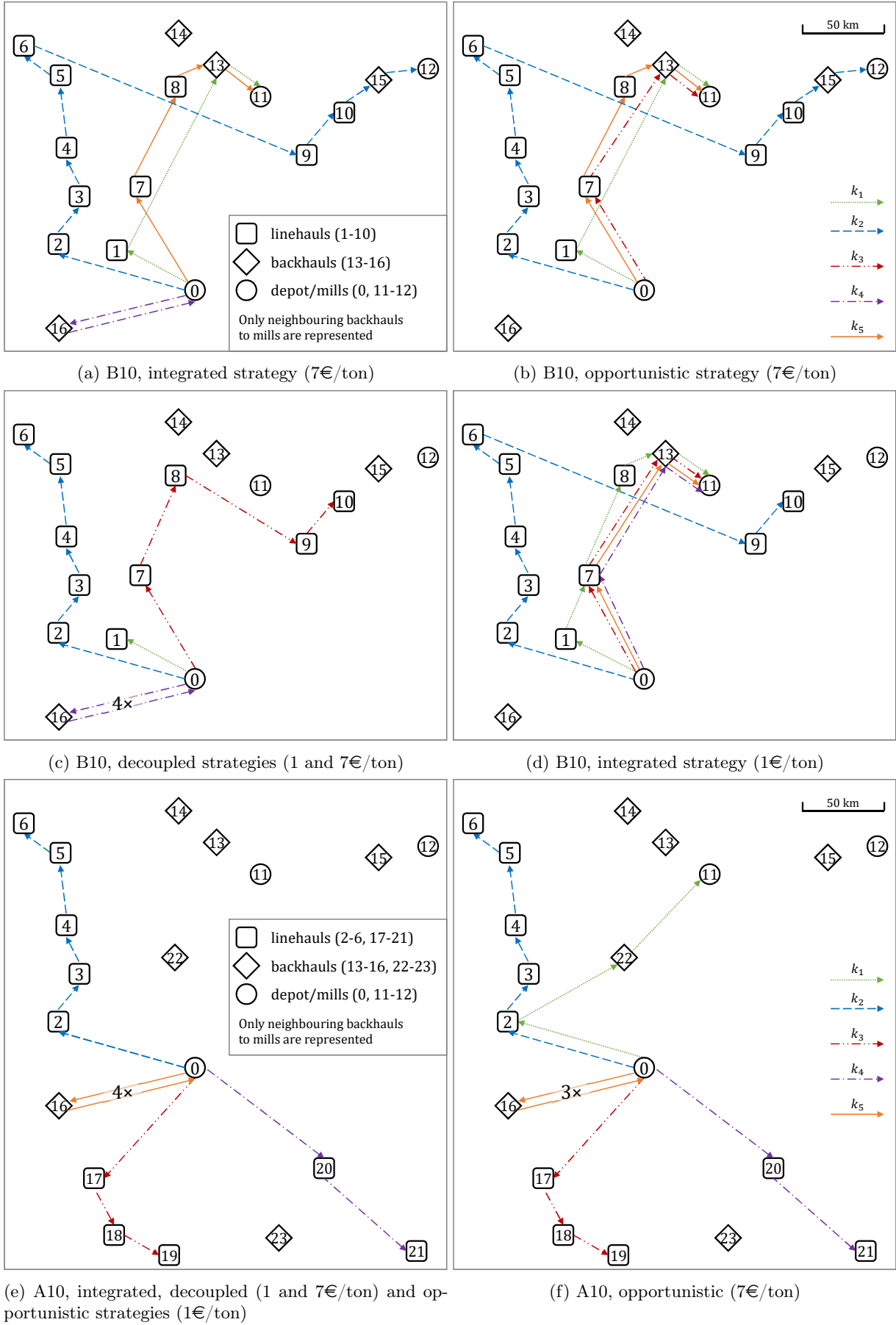
Figure 4: Graphical representation of the planning strategies for instances A10 and B10
