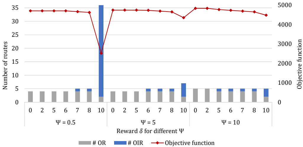
Figure 5: Impact of the variation of the reward ( \delta ) and minimum delivery ( \psi ) ( \alpha = 1,200, \beta = 0 )
