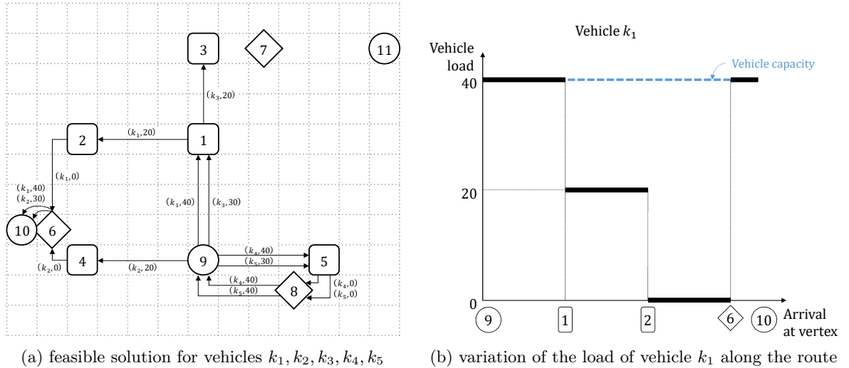
Figure 3: Example of a feasible solution for a rVRPB
