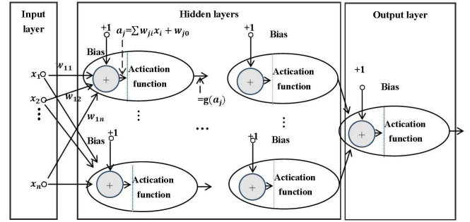
Fig. 6. The structure of the MLP.
