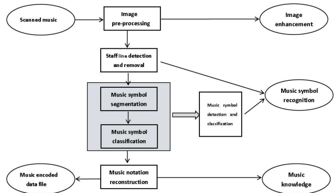
Fig. 1. Proposed architecture of the OMR system.
