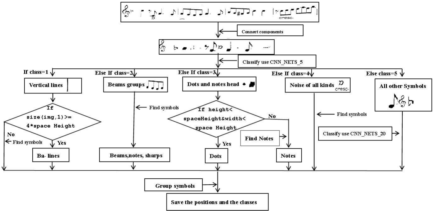
Fig. 7. The processing flow of the music symbol detection
