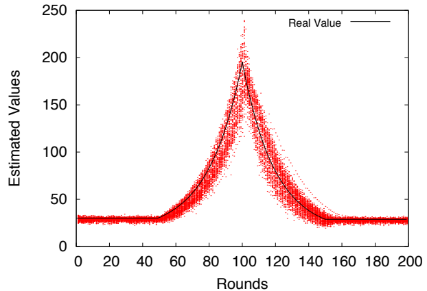
Fig. 5 Estimated value over rounds in a 1000 node 5000 link Erdos-Renyi network, with changes of the initial input value at 50% of the nodes.
