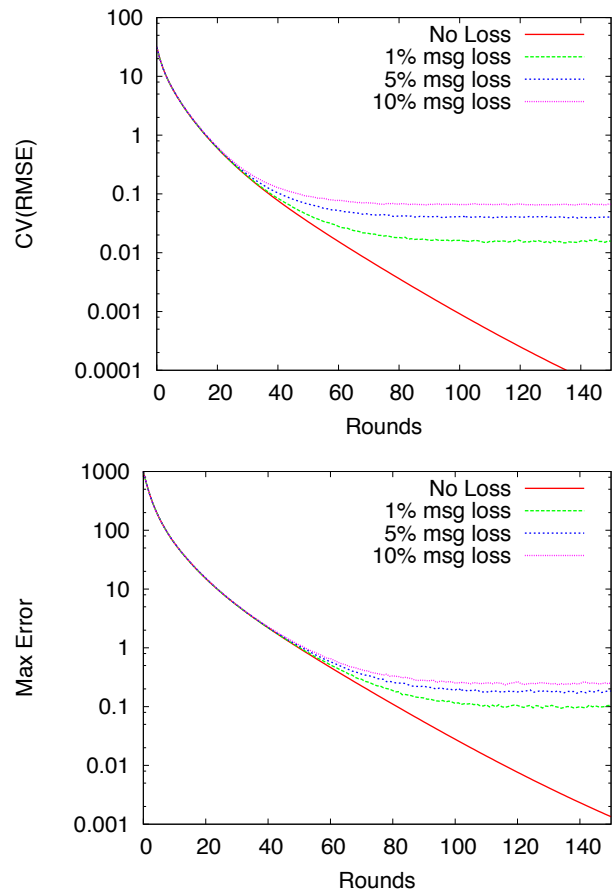
Fig. 2 Coefficient of variation of the RMSE and maximum relative error for MDFU in a 1000 node 5000 link Erdos-Renyi network.
