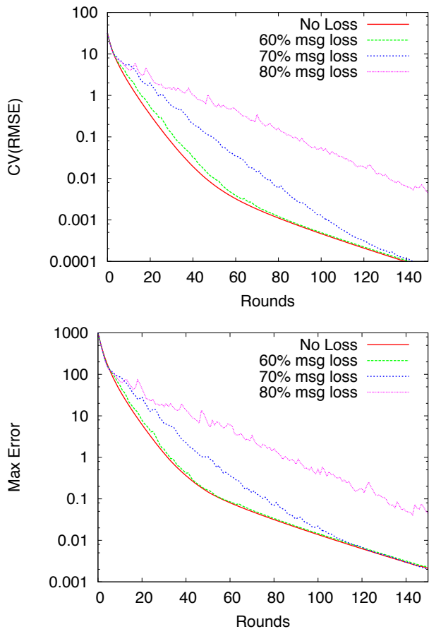
Fig. 4 Coefficient of variation of the RMSE and maximum relative error for MDFU-LP in a 1000 node 5000 link Erdos-Renyi network.
