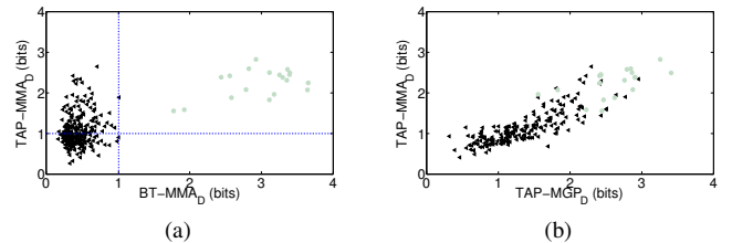
Figure 6: TAP-MMA_D and TAP-MGP_D for annotated 217 files in Dataset2. Pieces which are considered easy according to their BT-MMA_D are depicted by gray circles. (a): Scatter plot of TAP-MMA_D versus BT-MMA_D , dotted lines indicate the chosen border for difficult files for beat tracking (vertical line) and human tappers (horizontal line) (b): Scatter plot of TAP-MMA_D versus TAP-MGP_D
