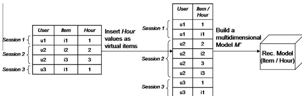
Fig. 1. Illustration of the learning process using the DaVI approach.
