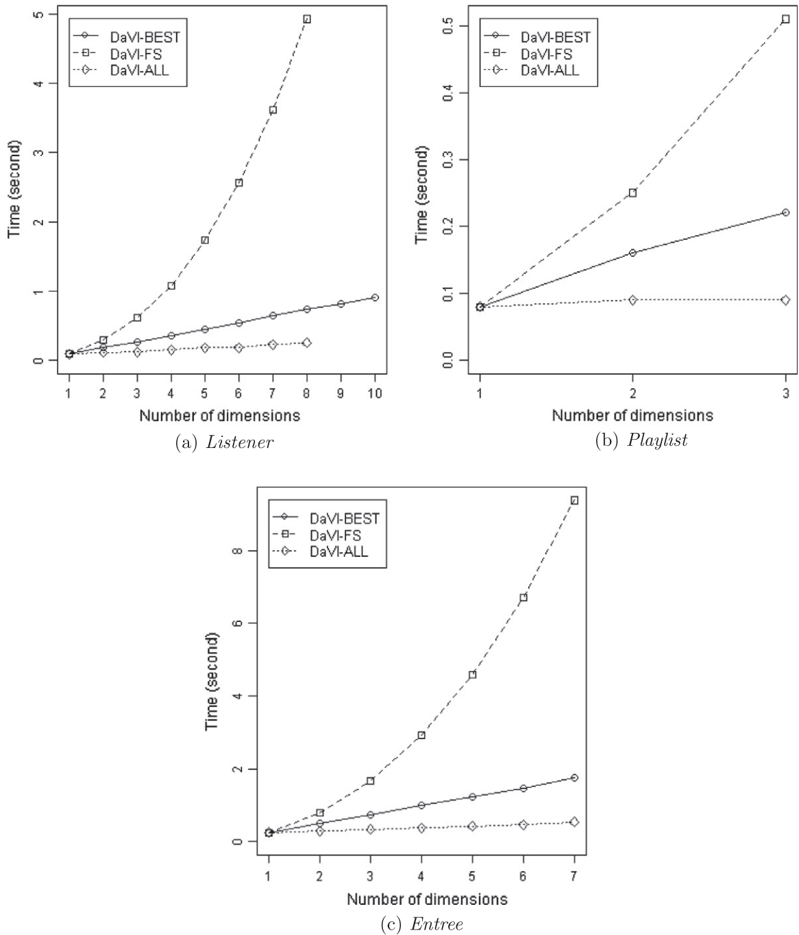
Fig. 6. Scalability of the DaVI-BEST , DaVI-FS and DaVI-ALL algorithms, using the AR technique, with respect to the number of dimensions.
