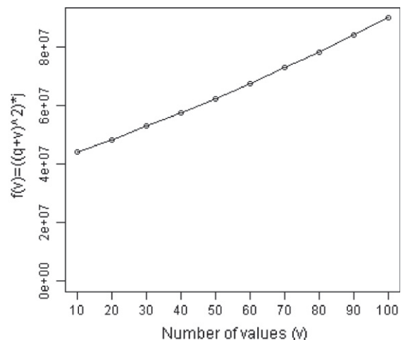
(b) q = 200 and j = 1000
