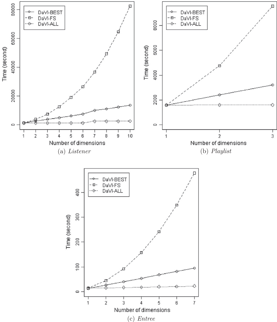
Fig. 5. Scalability of the DaVI-BEST, DaVI-FS and DaVI-ALL algorithms, using the CF technique, with respect to the number of dimensions.
