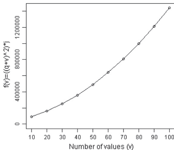
(a) q = 20 and j = 100
