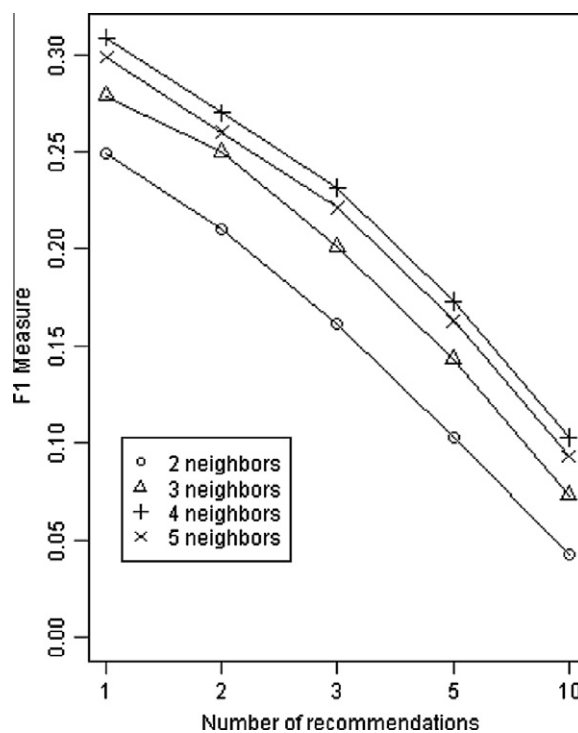
Fig. 4. Analyzing the DaVI-BEST algorithm using the CF technique with different number of neighbors in the Listener data set.
