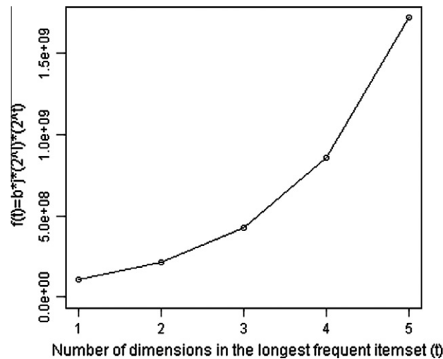
Fig. 3. Computational behavior of the DaVI approach using AR technique ( b = 14 , \ell = 7 and j = 30,000 ).
