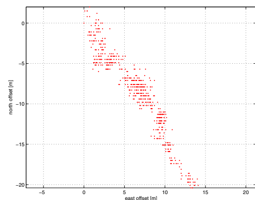
Fig. 6. NIB motion relative to the initial position.
