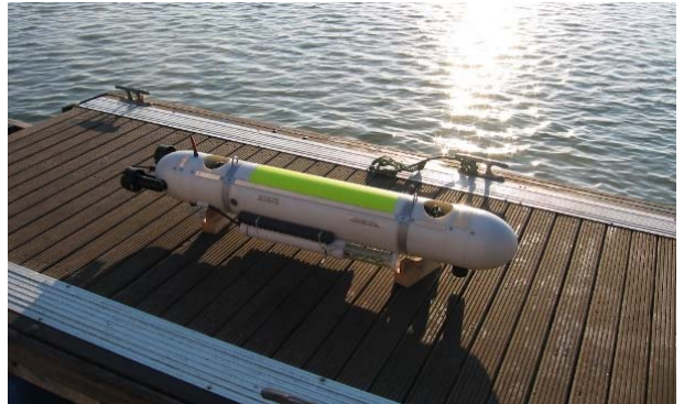
Fig. 1. MARES AUV with an external CTD.
