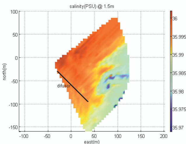
Fig. 9. Salinity map close to the sewage outfall diffuser.
