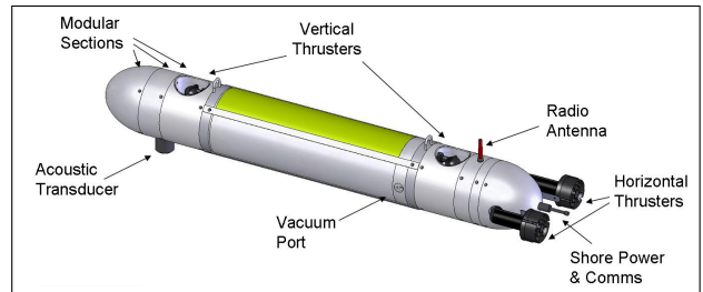
Fig. 2. MARES Solidworks® model.
