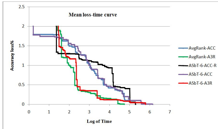
Fig. 2. Loss-time curves for sample-based active testing and average ranking methods, accuracy-based and A3R-based versions ( N = 64 ).
