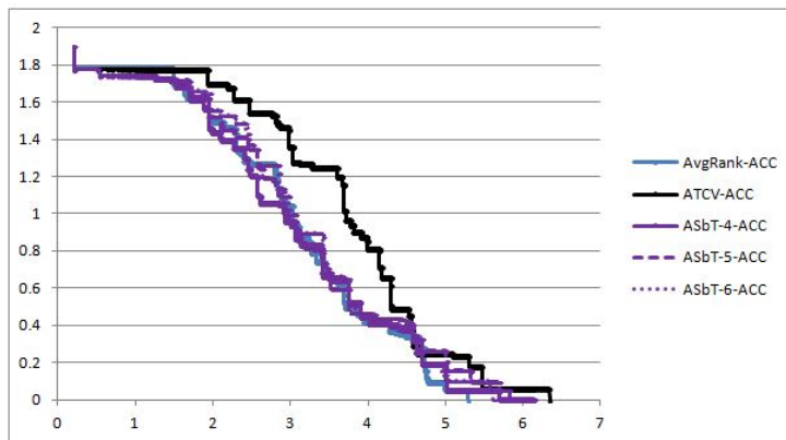
Fig. 1. Mean loss-time curves for 3 variants of ASbT (using sample number 4, 5 and 6), ACTV-ACC and the average ranking method (AvgRank-ACC).
