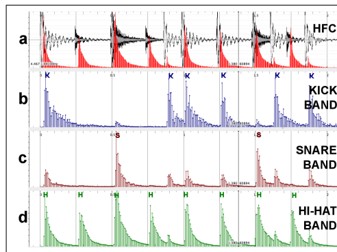
Fig. 2. a) The audio signal and the HFC onset detection function values; b),c),d) The complex onset detection functions values for each drum class, as a part of the event detection and instance filtering stage.
