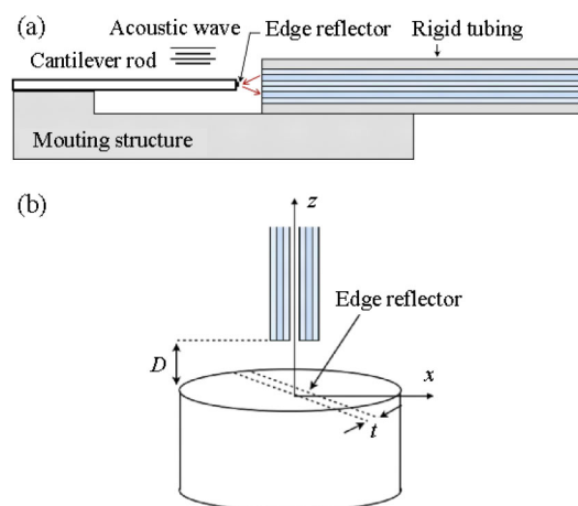
Fig. 6 Sensing configuration demonstrated in [40] for a two-fiber optical probe with the cantilever for acoustic wave detection.
