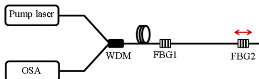
Fig. 11 Sensing configuration based on a DBR fiber laser (adapted from [54]).
