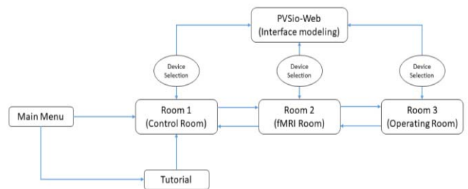
Figure 2: Game flowchart.
