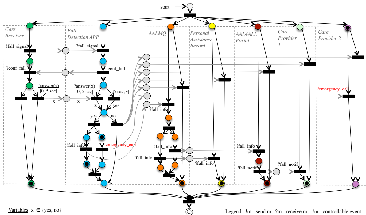
Figure 4: TEDCPN derived from the SD of Figure 3. The net is marked in a final state of a failed test execution in which the fall detection application didn't send an emergency call.
