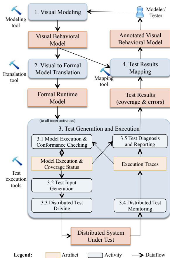
Figure 1: Dataflow view of the proposed test process.
