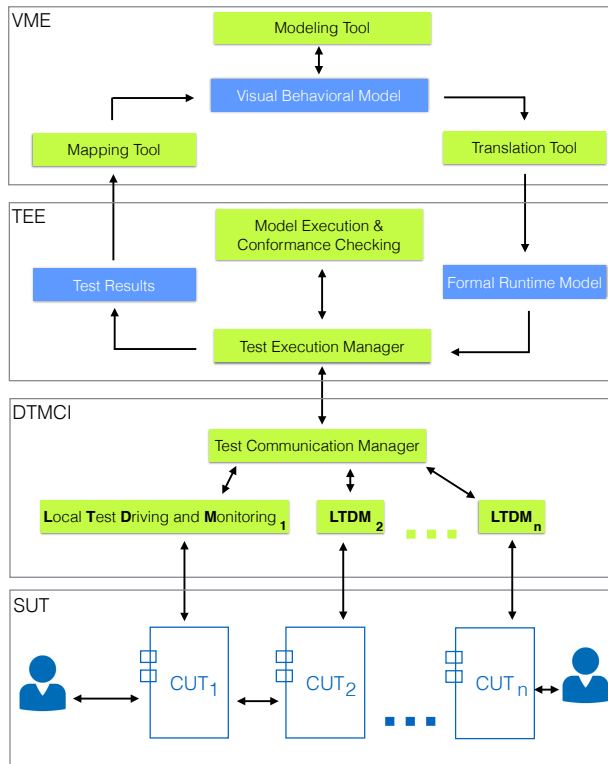
Figure 5: Toolset architecture.
