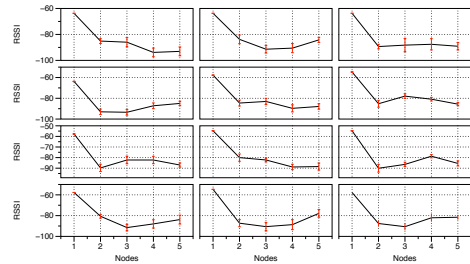
Fig. 15. Fingerprint for Lr-Wpan network for a dry soil.
